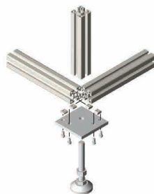
Mounting Example Mounting of Leveling Mounts
