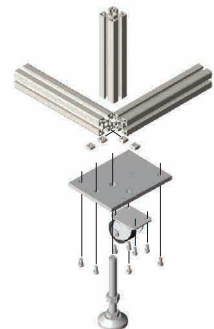
Mounting of the Leveling Mount + Plate with Caster
