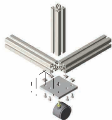
Mounting of Plate with Caster
