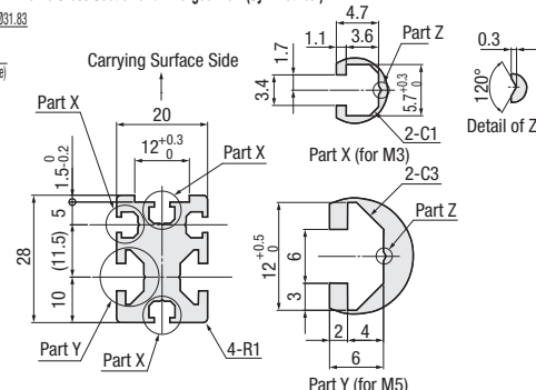
Frame Cross Section and Enlarged View (Symmetrical)
