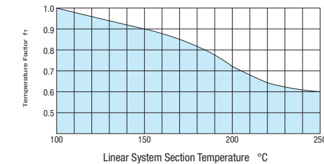
Fig. Temperature Coefficient
